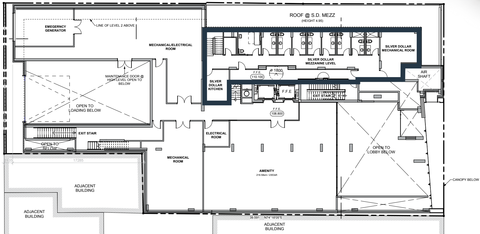
Second Floor - 2,411 SF
